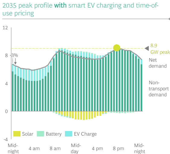
Exhibit 63: Smart charging and Time of Use pricing can reduce peak demand by 1.9 GW
