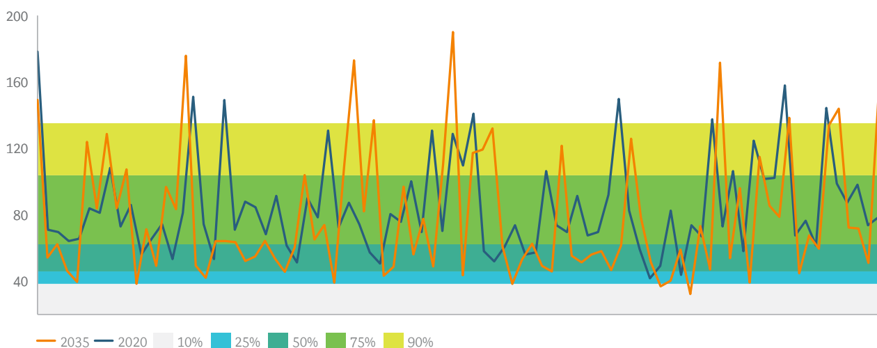
2020 current system vs 2035 100% renewable pathway annual price distribution $/MWh
