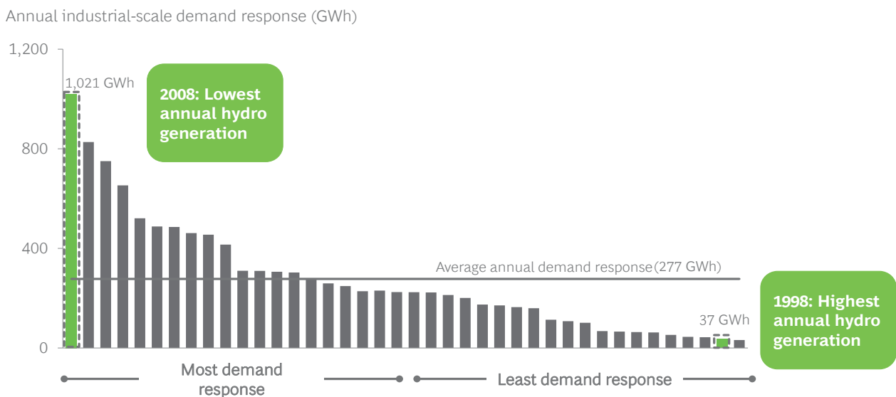
Exhibit 87: 2030 industrial-scale demand response for 40 hydrological years
