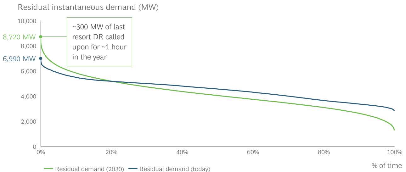
Exhibit 82: 2030 residual demand duration curve
