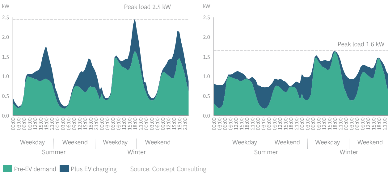
Exhibit 100: Household demand contribution from an electric vehicle
