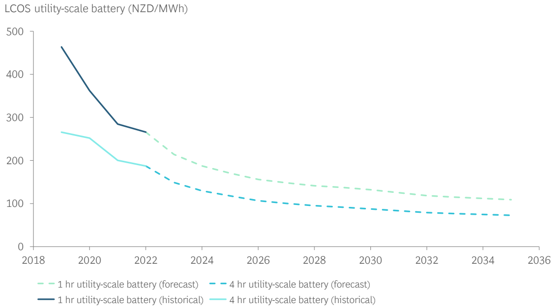
Exhibit 27: Historical and forecast declines in levelised cost of storage
